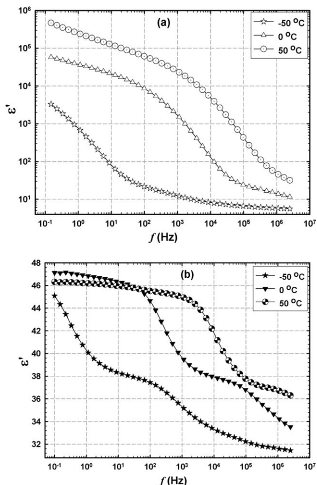
Figure 3. Frequency dependence of \epsilon' for (a) C_{60}(OH)_{29} and (b) Sc_3N@C_{80}(OH)_{18} samples at three temperatures.
