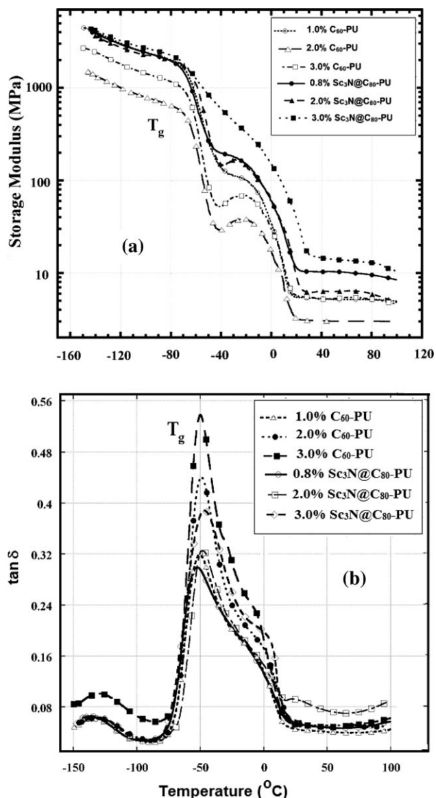
Figure 1. (a) Dynamic storage modulus ( E' ) and (b) loss tangent ( \tan \delta ) versus temperature for fullerene-PU compositions.
