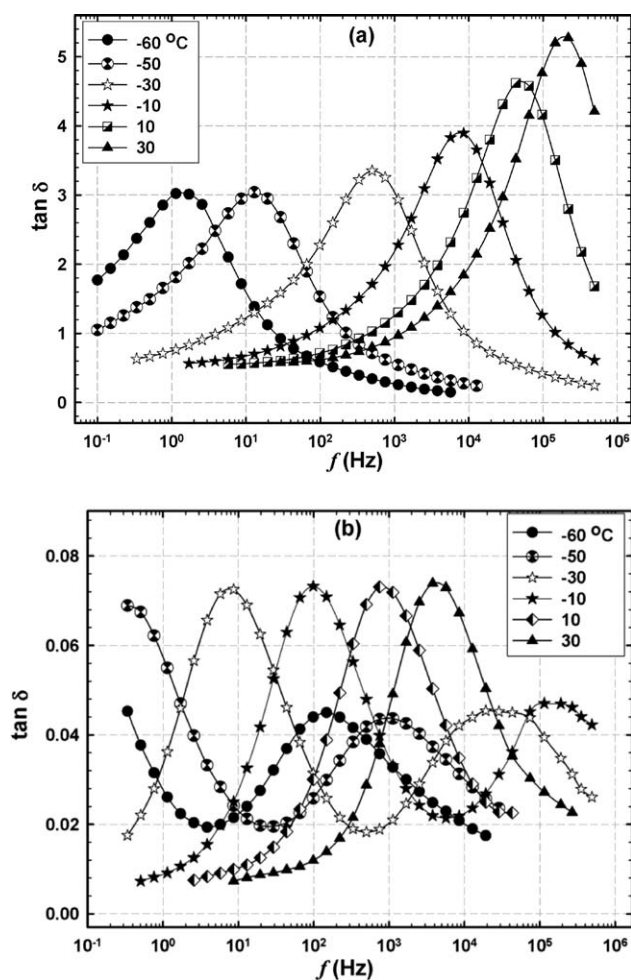
Figure 4. \tan \delta versus frequency at select temperatures for (a) C_{60}(OH)_{29} and (b) Sc_3N@C_{80}(OH)_{18} samples.
