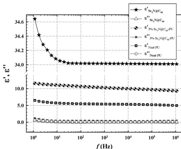
Figure 8. \epsilon' and \epsilon'' versus f for \text{Sc}_3\text{N}@C_{80} and 3% \text{Sc}_3\text{N}@C_{80} -PU versus Neat PU networks at 20^\circ\text{C} (data via Novocontrol BDS).
